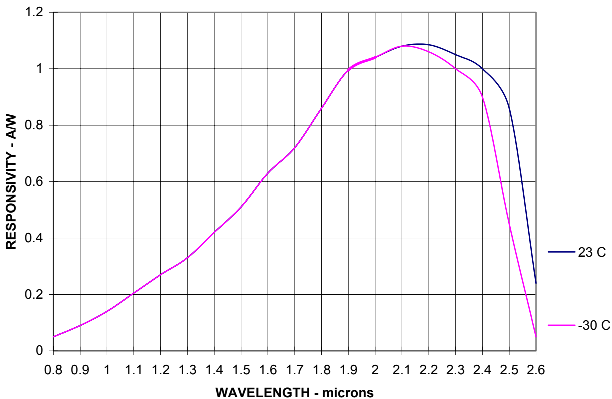
SPECTRAL RESPONSE - IGA2.2-series
