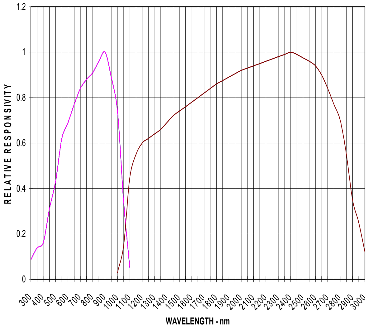
S/PBS 2-COLOR PHOTODETECTOR Typical Spectral Response - 22C
