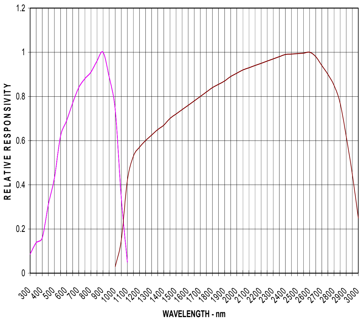
S/PBS 2-COLOR PHOTODETECTOR Typical Spectral Response - -30C
