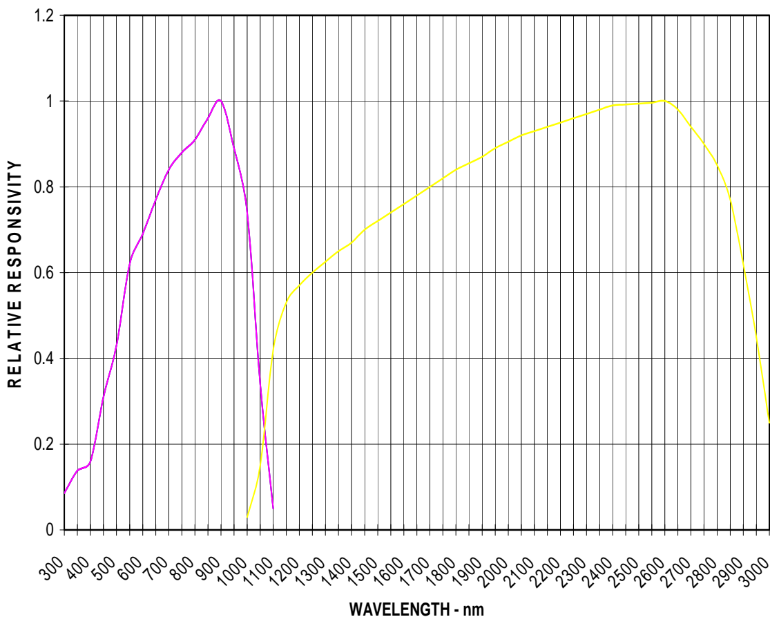
S/PBS 2-COLOR PHOTODETECTOR Typical Spectral Response - -30C
