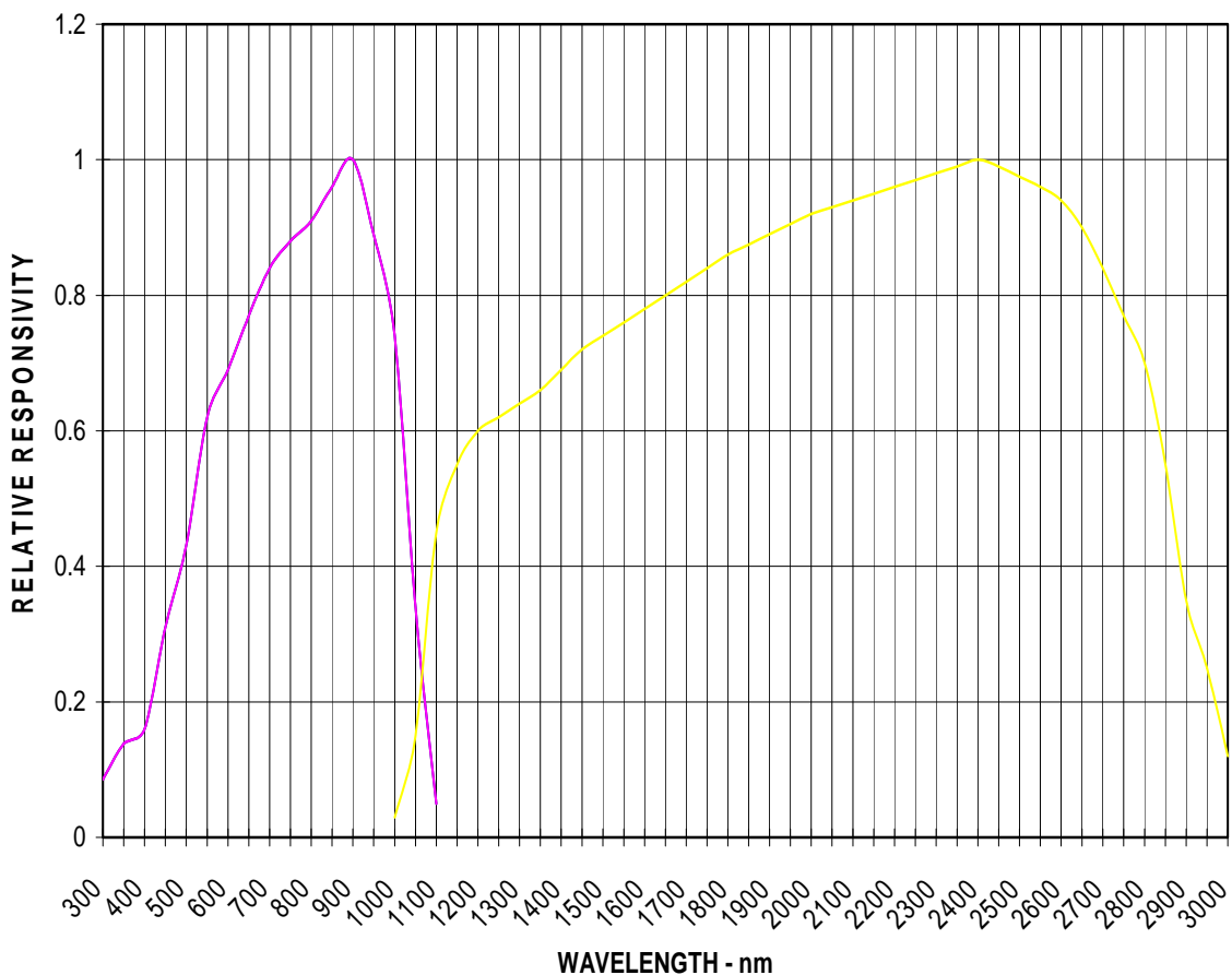
S/PBS 2-COLOR PHOTODETECTOR Typical Spectral Response - 22C
