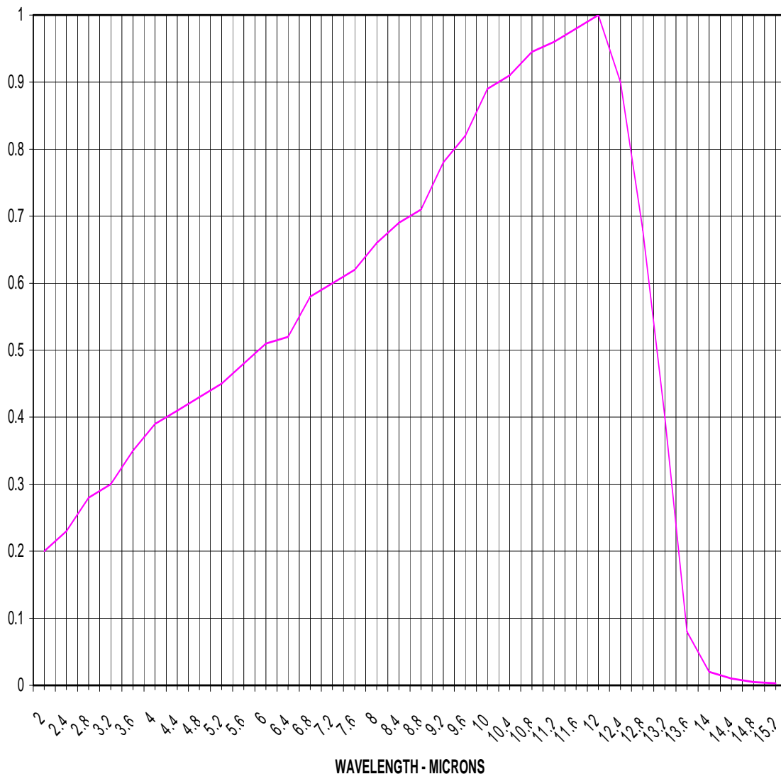
TYPICAL MCT(12) RELATIVE SPECTRAL RESPONSE
