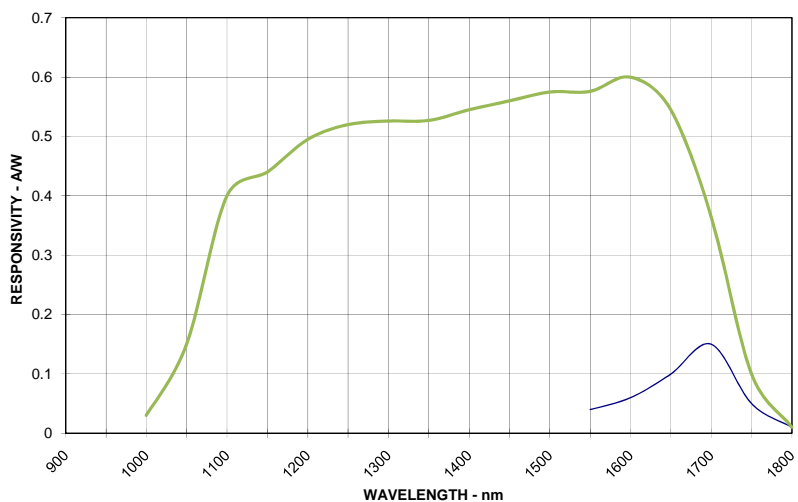
IGA/IGA-020 2-COLOR PHOTODIODE Typical Spectral Response - 22C
