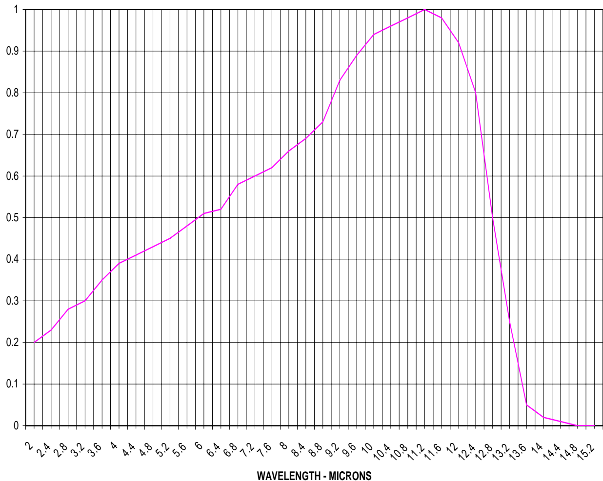
MCT10-series RELATIVE SPECTRAL RESPONSE
