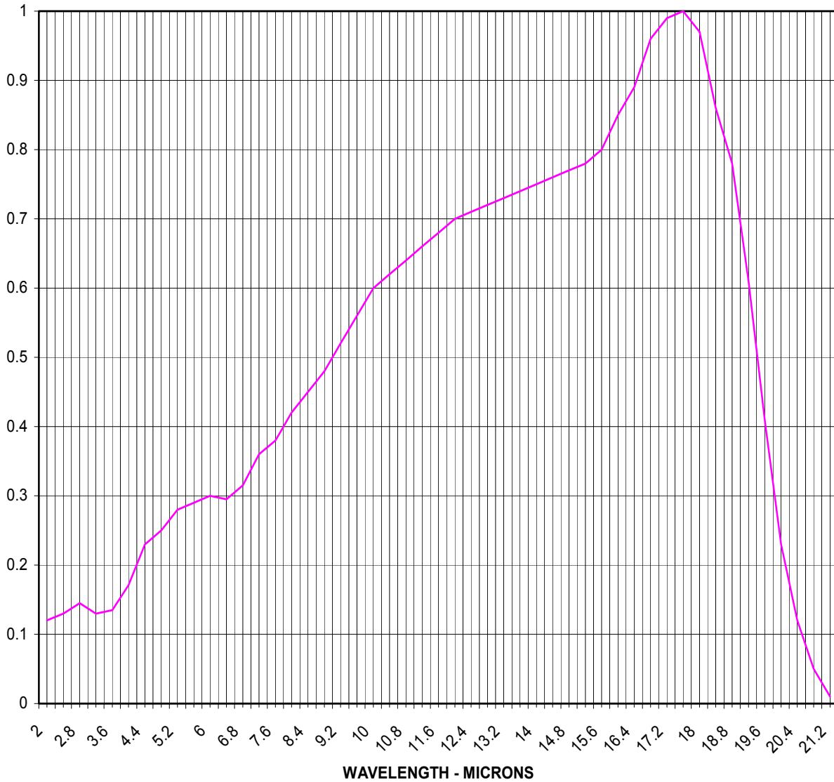
MCT RELATIVE SPECTRAL RESPONSE MCT20-Series, typical
