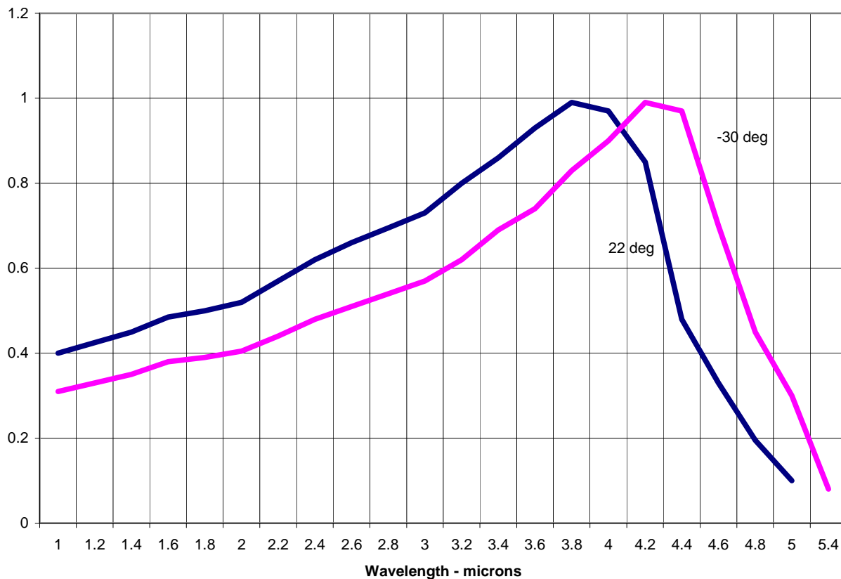
TYPICAL PBSE RELATIVE SPECTRAL RESPONSE
