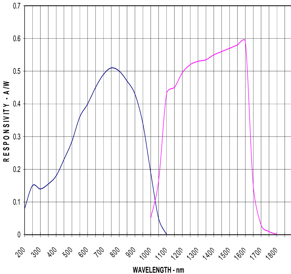
UVS/IGA 2-COLOR PHOTODIODE Typical Spectral Response : -30C
