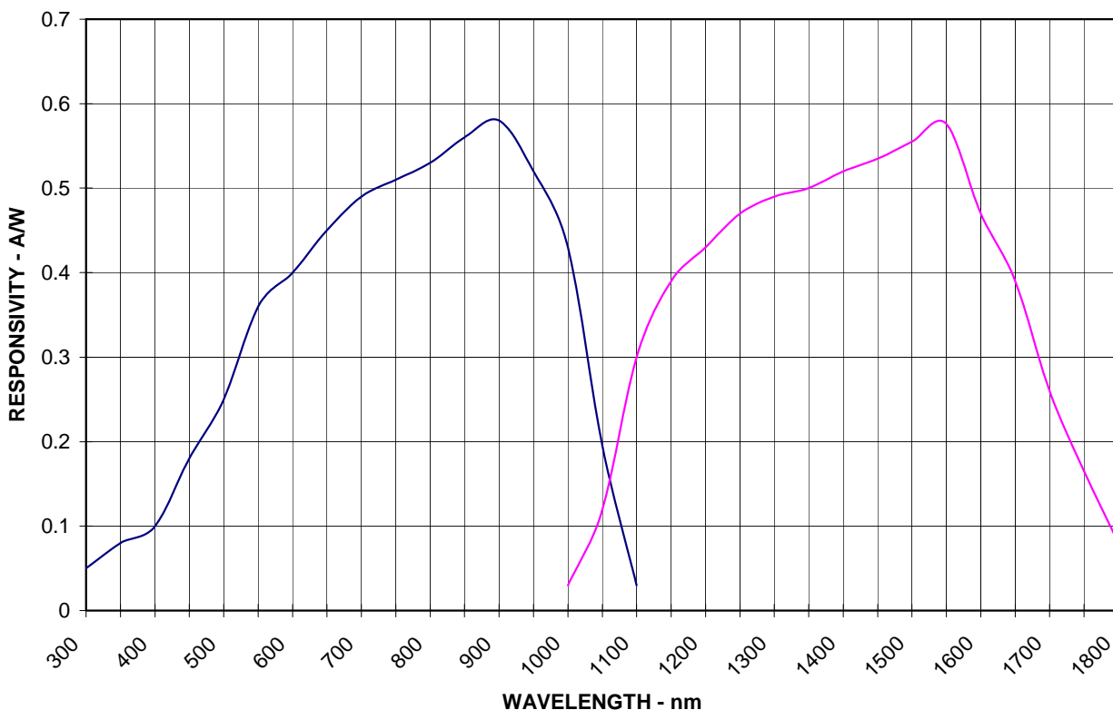
S/G 2-COLOR PHOTODIODE Typical Spectral Response - 22C
