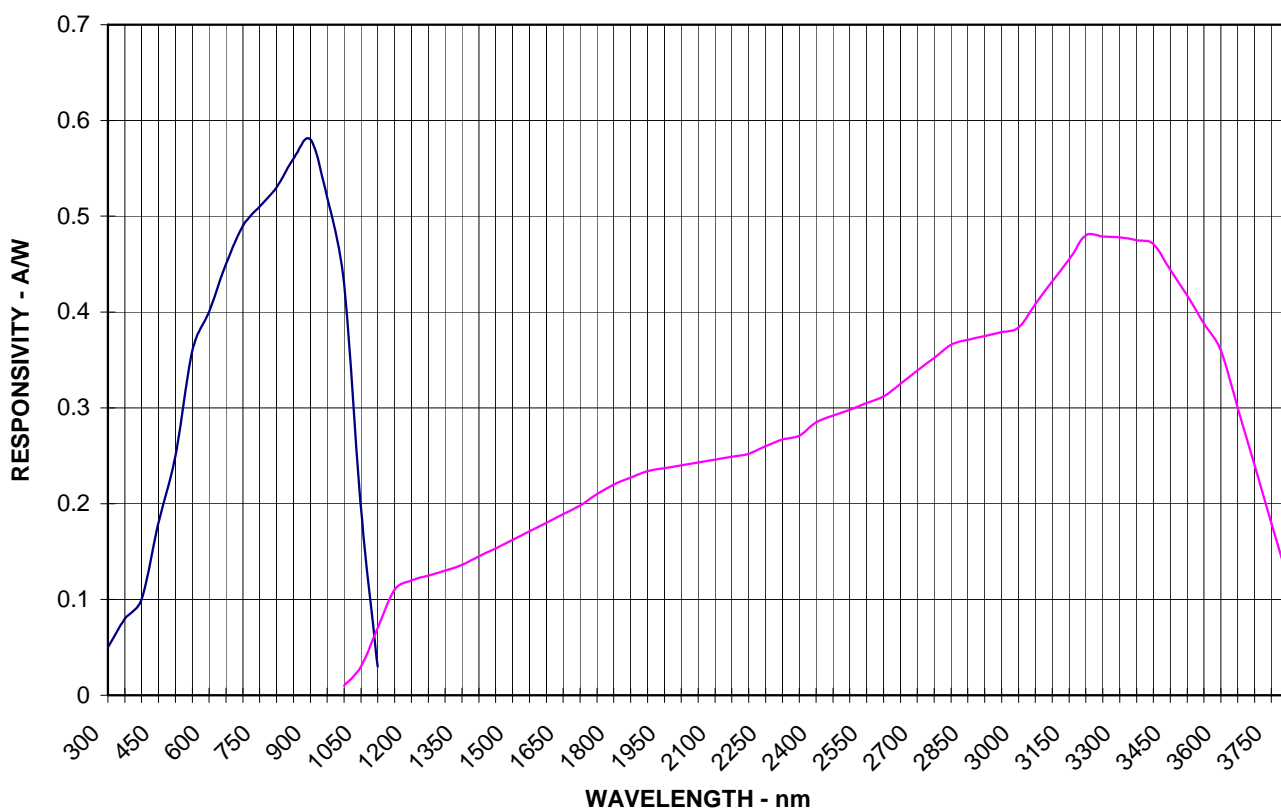
S/IA 2-COLOR PHOTODIODE Typical Spectral Response - 22C
