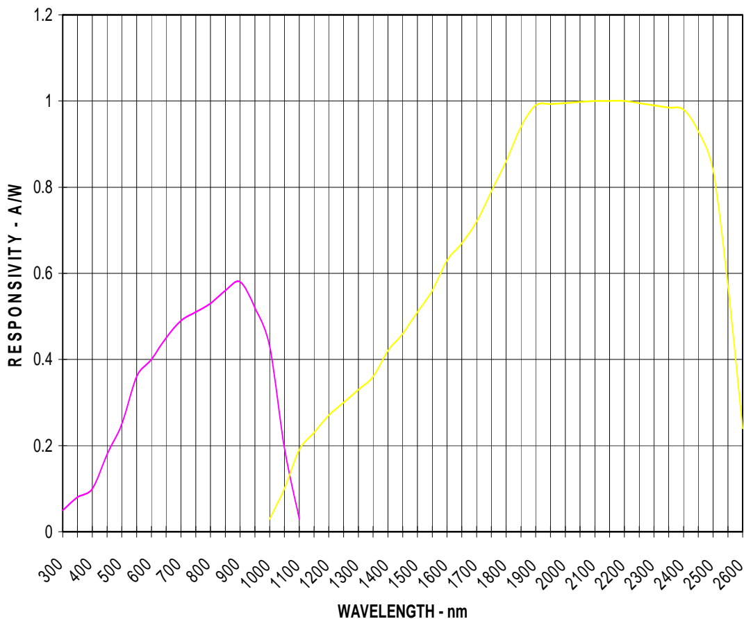
S/IGA2.2 2-COLOR PHOTODIODE Typical Spectral Response - 22C
