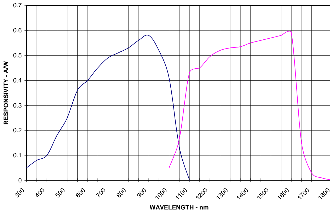
S/IGA 2-COLOR PHOTODIODE Typical Spectral Response : -30C
