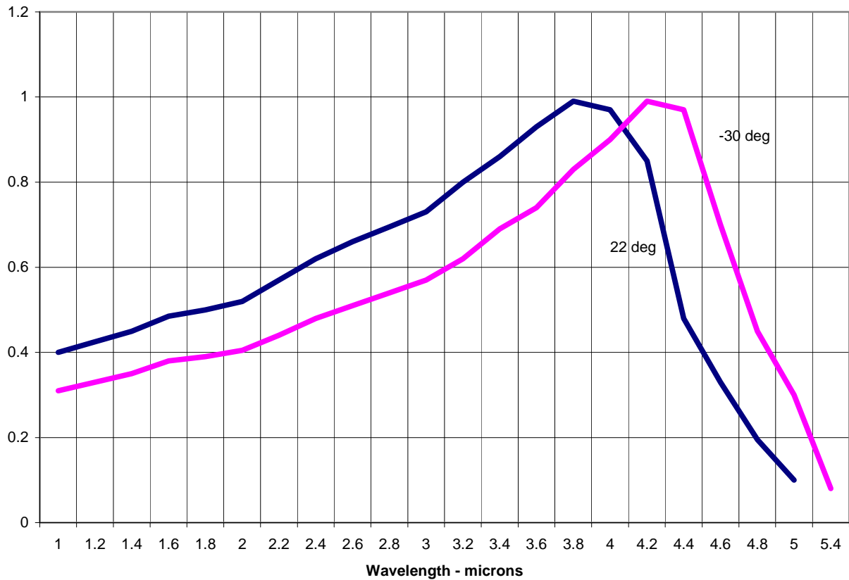
TYPICAL PBSE RELATIVE SPECTRAL RESPONSE
