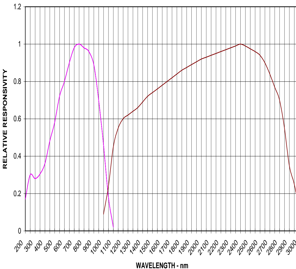
UVS/PBS 2-COLOR PHOTODETECTOR Typical Spectral Response - 22C
