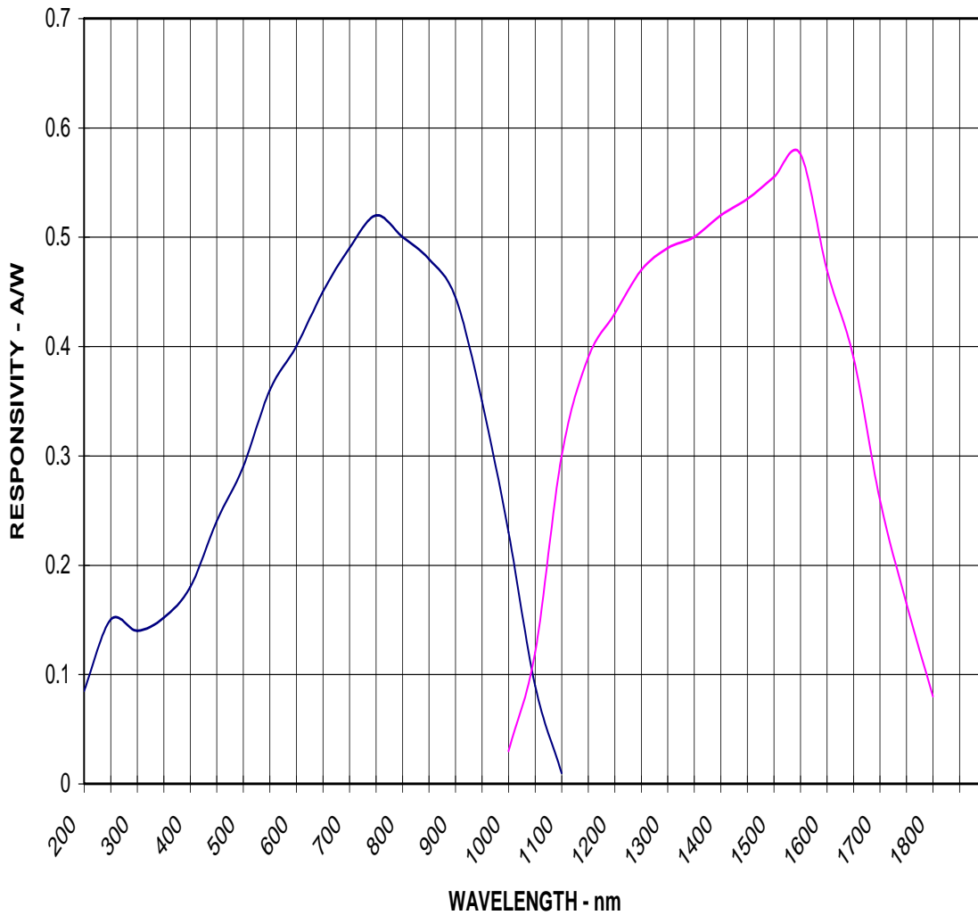
UVS/G 2-COLOR PHOTODIODE Typical Spectral Response - 22C
