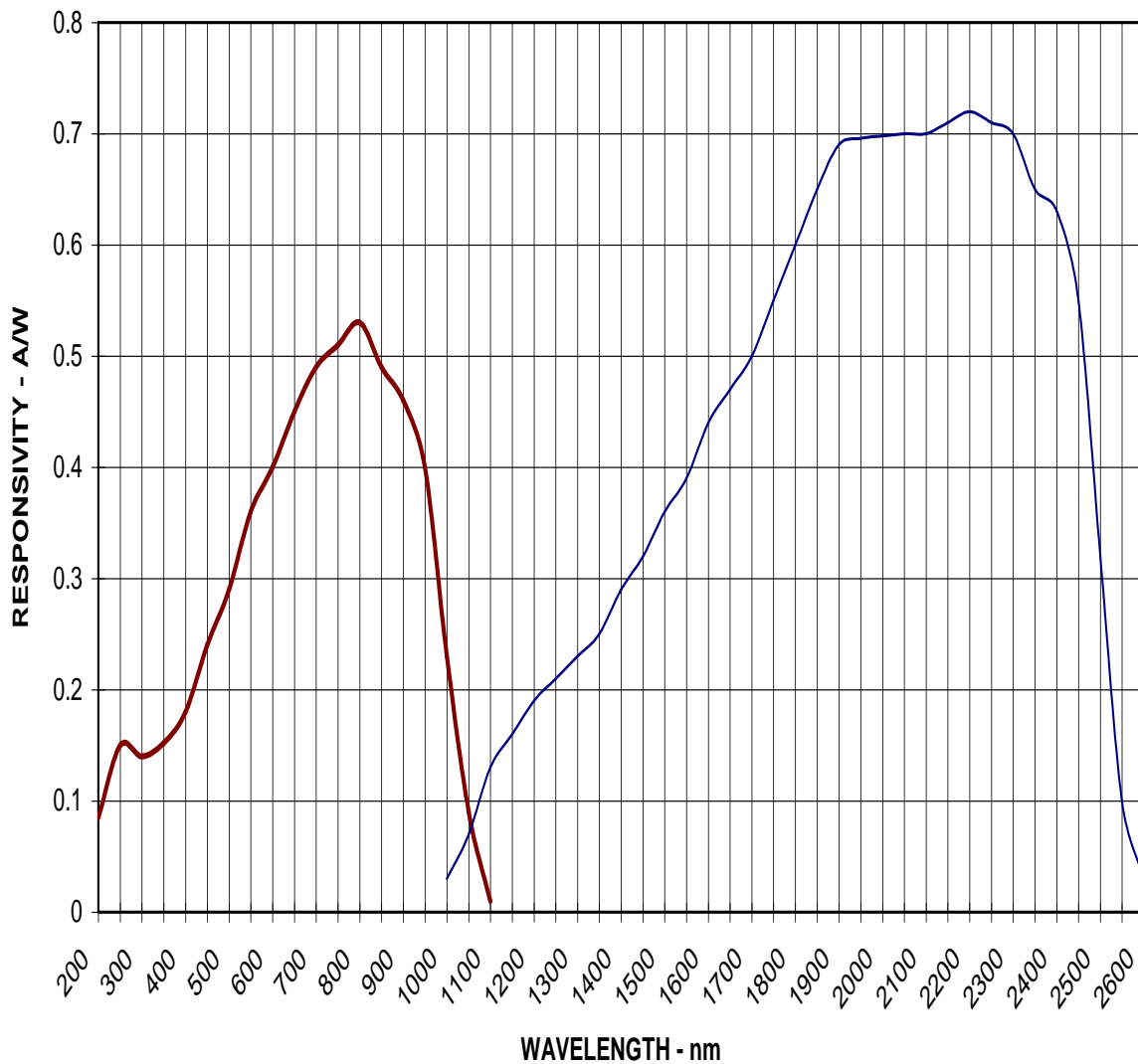
UVS/IGA2.2 TC 2-COLOR PHOTODIODE Typical Spectral Response - -30C
