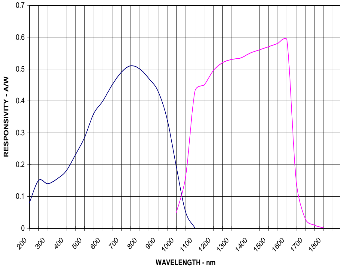
UVS/IGA 2-COLOR PHOTODIODE Typical Spectral Response : -30C
